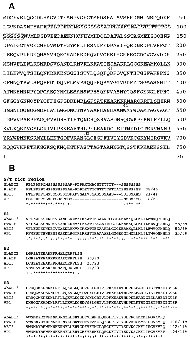
Fig. 1 The deduced amino acid sequence of WbABI3 . (A) An N-terminal serine domain and three basic domains (B1-B3) conserved in ABI3 / VP1 like factors are shaded and underlined, respectively. (B) Sequence comparison of the conserved domains between WbABI3, PvALF (French bean), ABI3 ( Arabidopsis ) and VP1 (maize). Alignments were performed by T-coffee program. The numbers of identical amino acids/total amino acids in each domain of PvALF, ABI3 and VP1 to WbABI3 are indicated.
